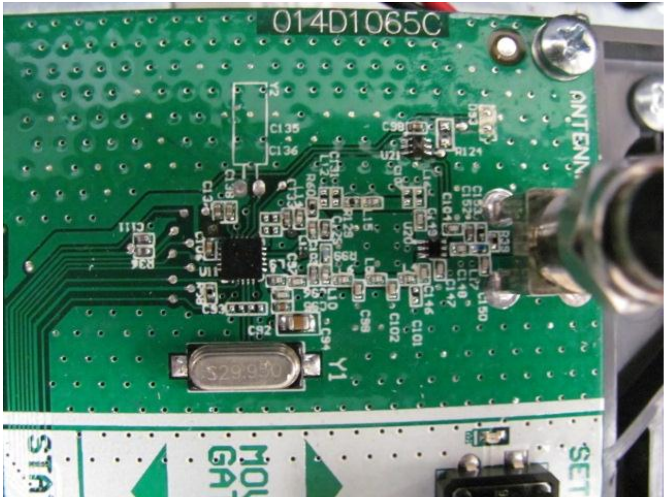
RF Section
