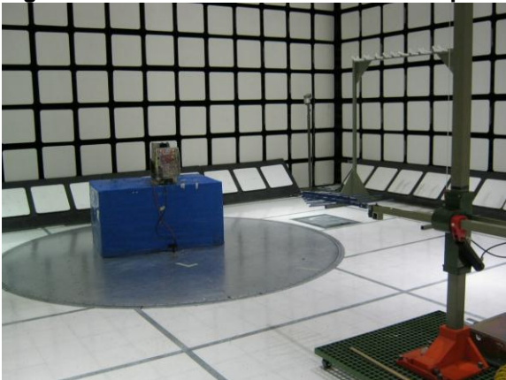
Figure 35 Radiated Emissions Test Setup
