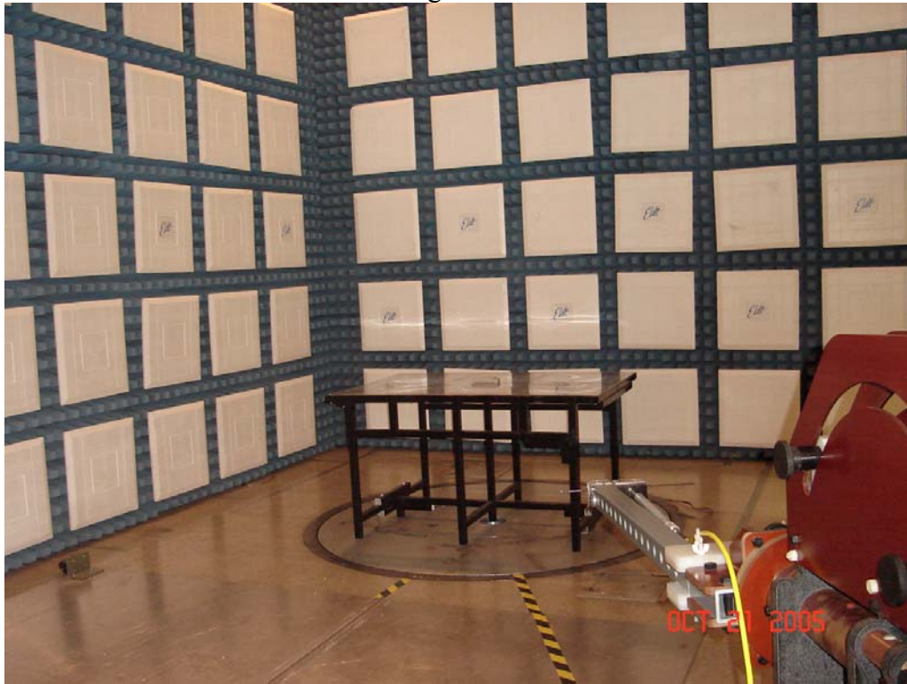
Test Setup for Radiated Emissions, 390MHz - Horizontal Polarization
