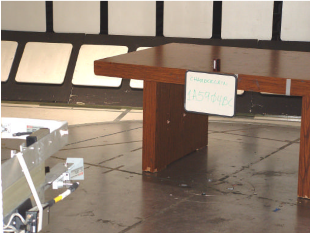
3m above 1GHz setup
