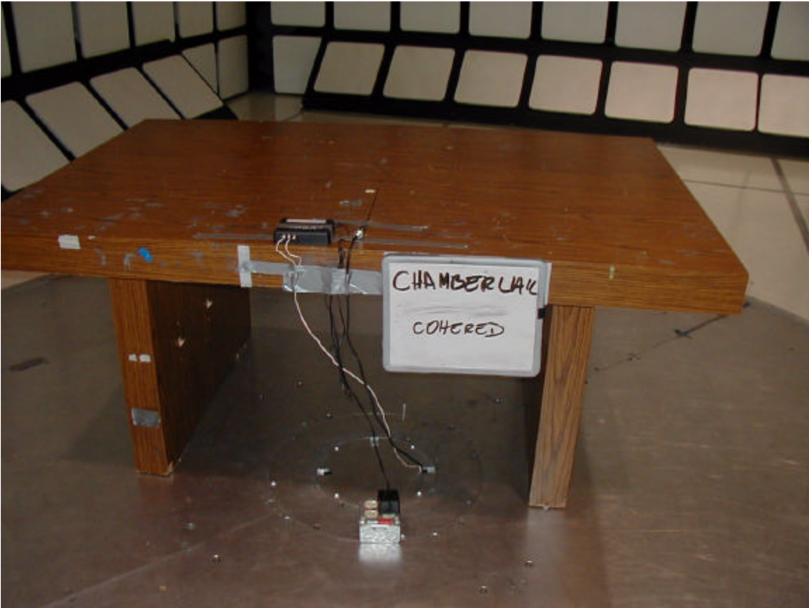
Radiated Emissions Test Setup Photos for 535-315LM
