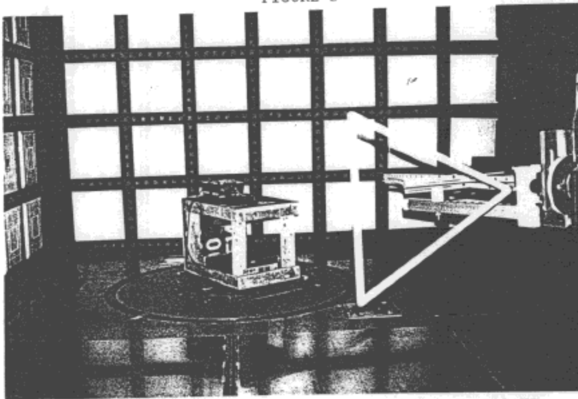
TEST SETUP FOR MEASUREMENT OF RADIATED EMISSIONS HORIZONTAL POLARIZATION
