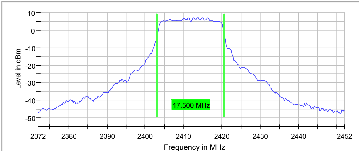
99 % Bandwidth
