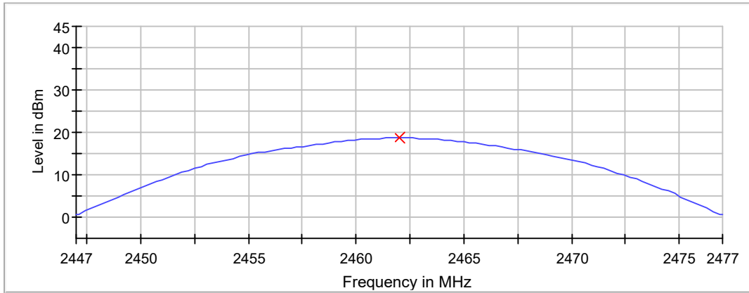
Peak Power
