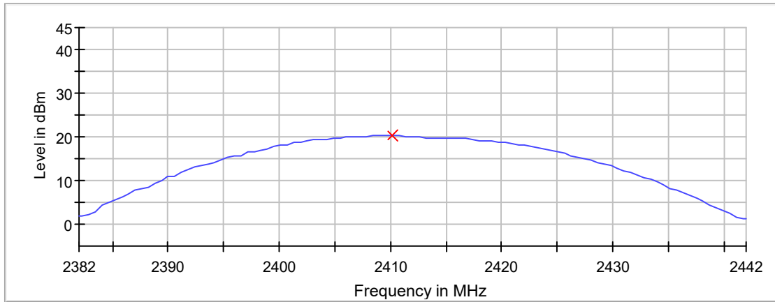
Peak Power
