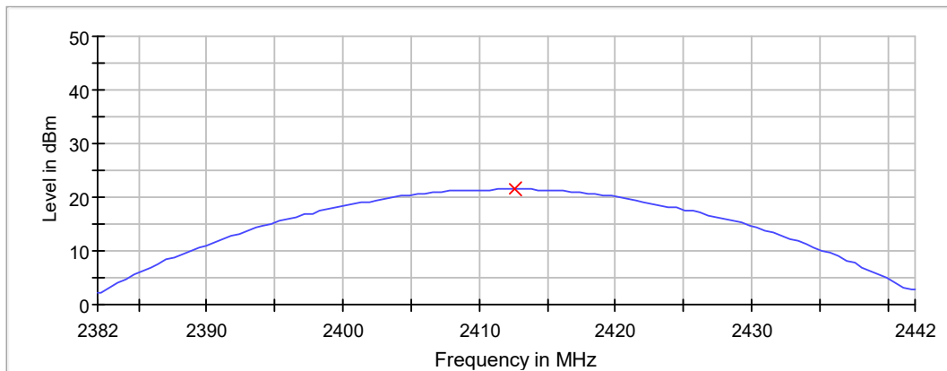
Peak Power
