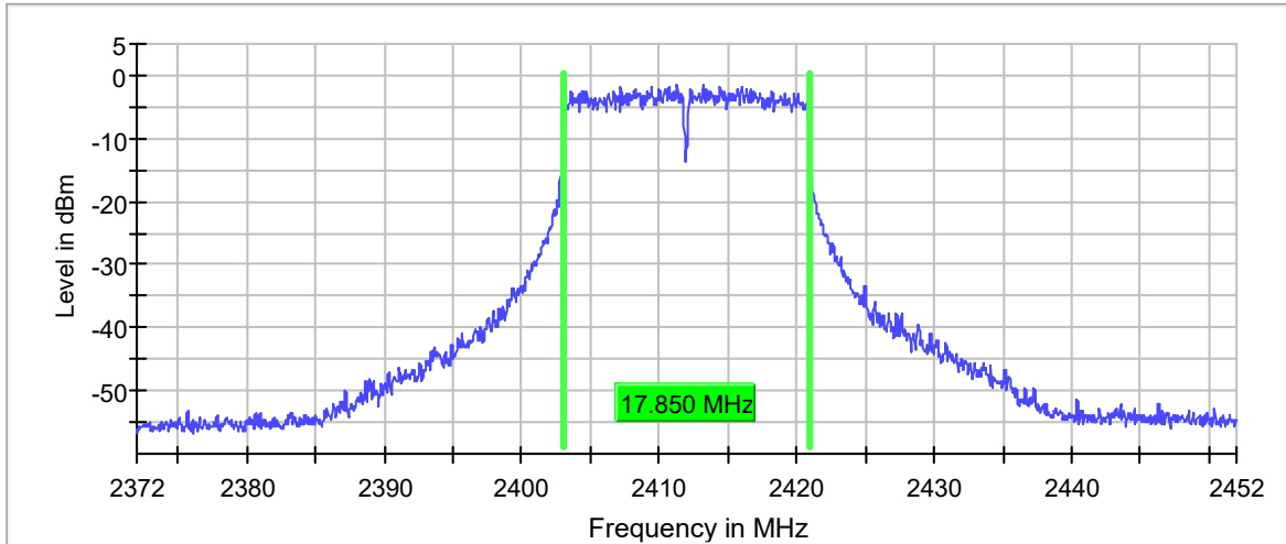
6 dB Bandwidth
