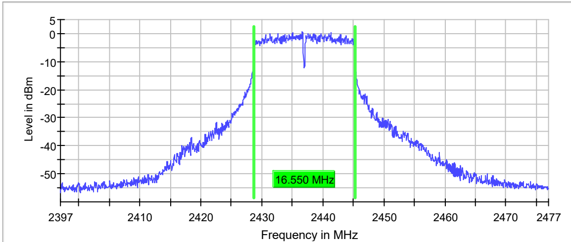
6 dB Bandwidth
