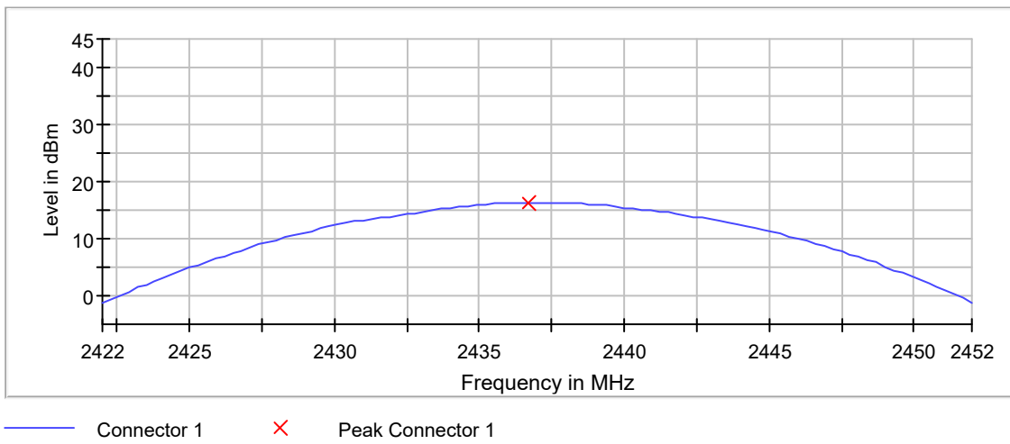
Peak Power
