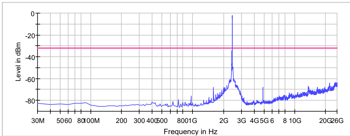
Spurious
