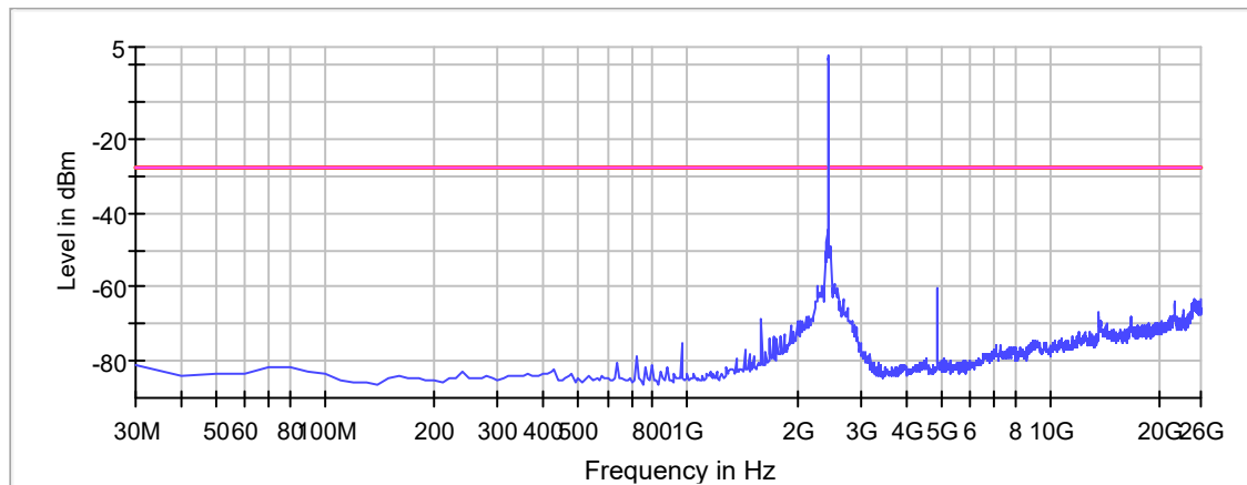
Spurious
