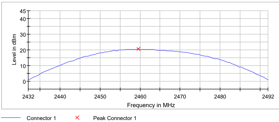
Peak Power
