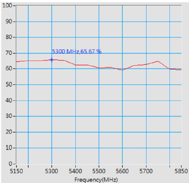
Maximum Efficiency at 5300 MHz : 65.67 %
