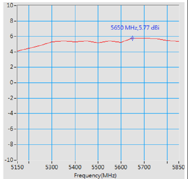
Maximum Peak Gain at 5650 MHz : 5.77 dBi
