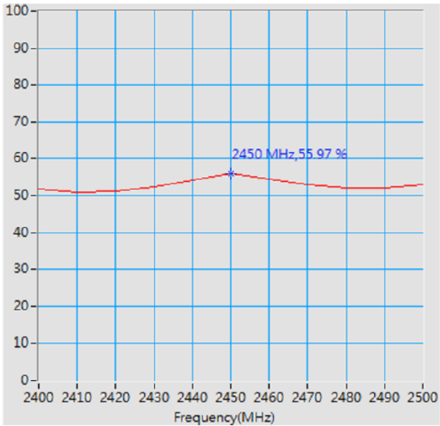
Maximum Efficiency at 2450 MHz : 55.97 %
