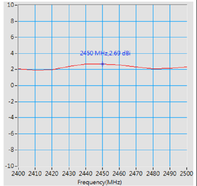
Maximum Peak Gain at 2450 MHz : 2.69 dBi
