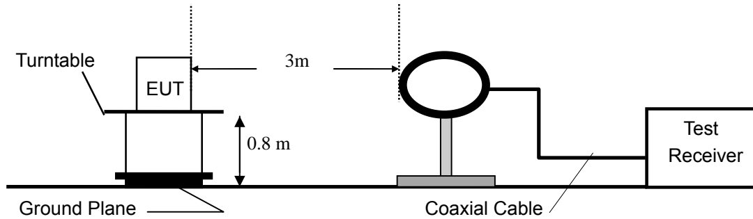
Radiated Emission Test Set-Up, Frequency Below 30MHz
