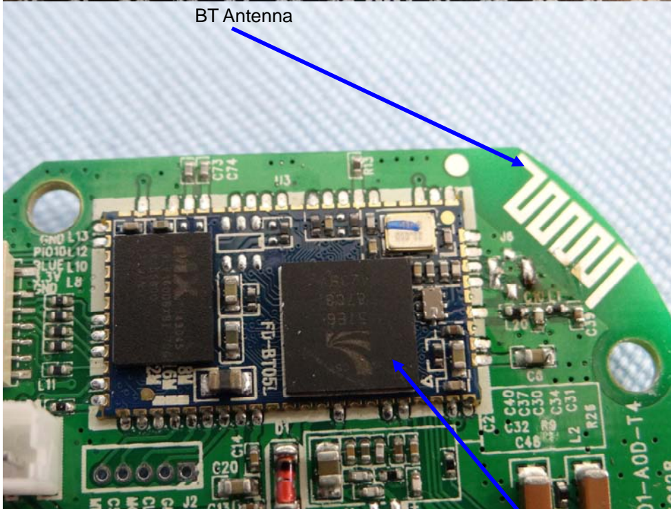
BT Chip
