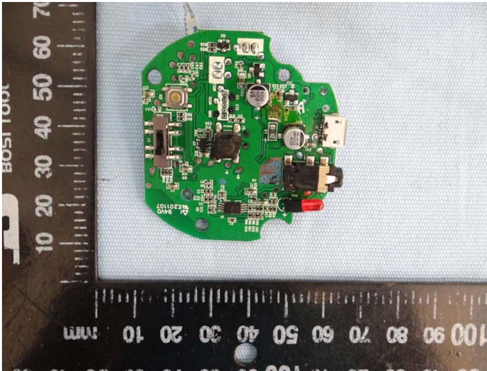
BT Antenna
