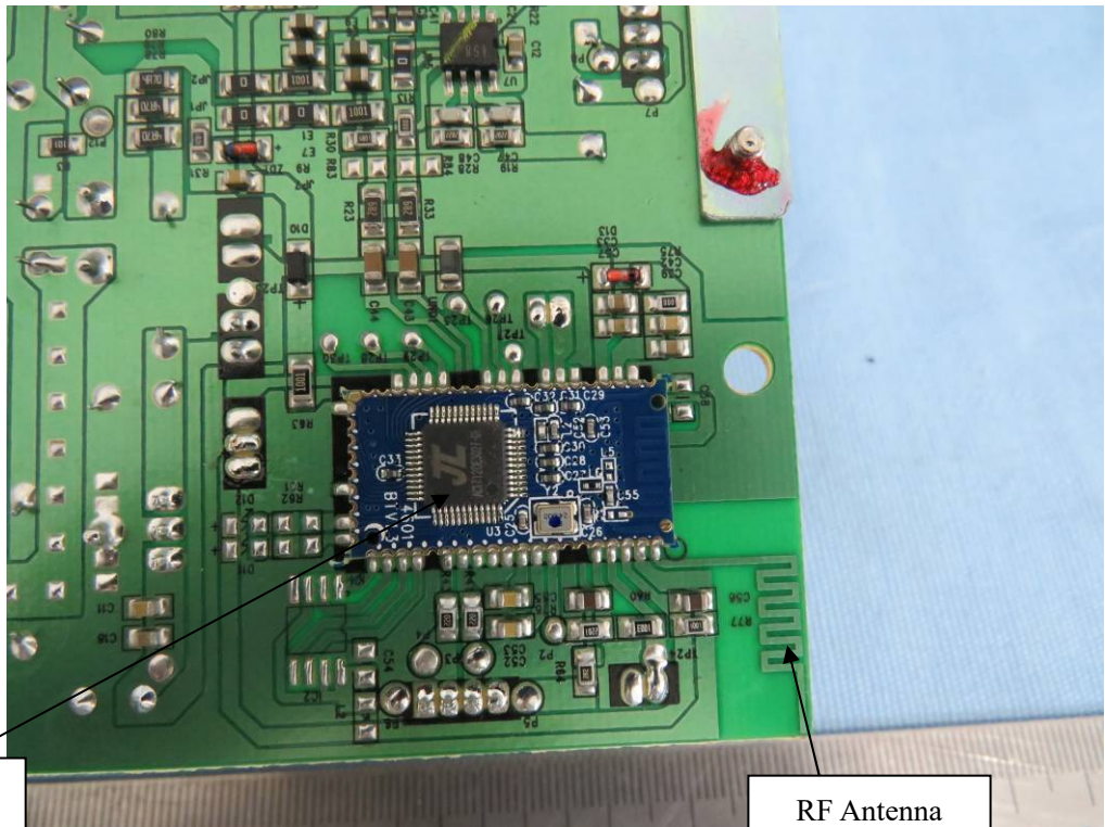
RF Chip
