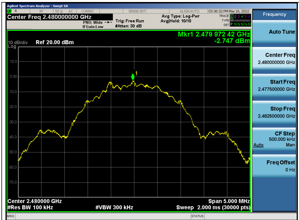
Test_Graph_LE2M_ANT1_2480_2Mbps_Reference Level
