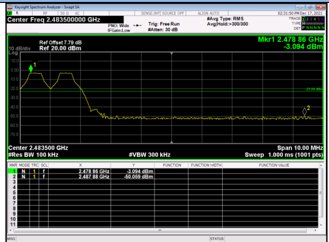
GFSK / Hopping
