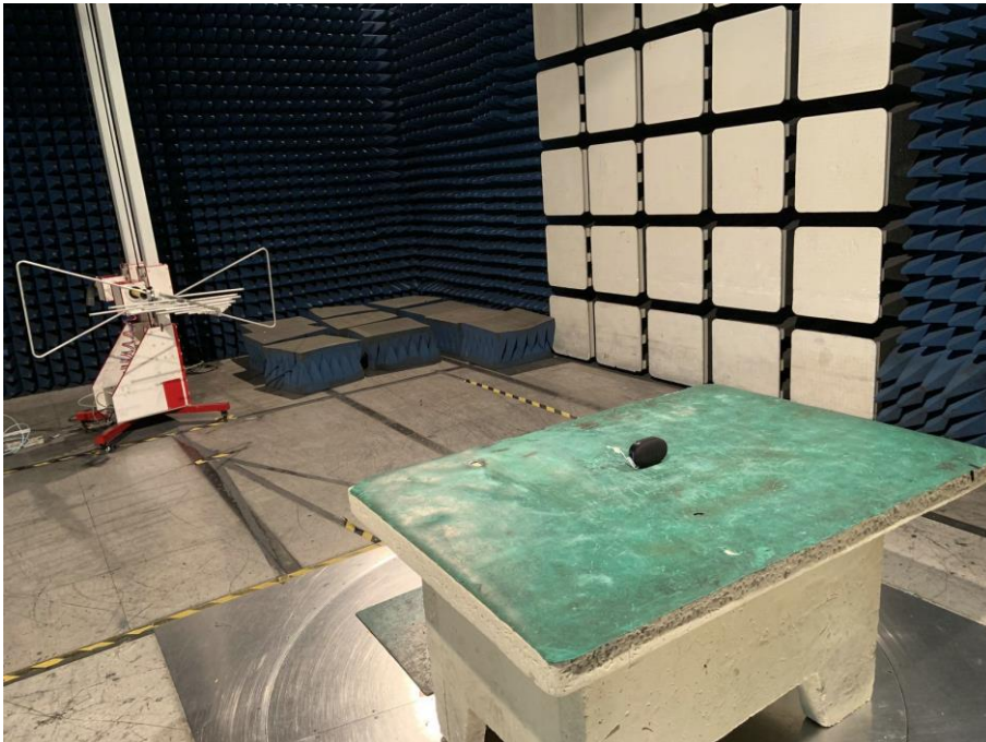
Setup Photos for Radiated Spurious Emission below 1GHz
