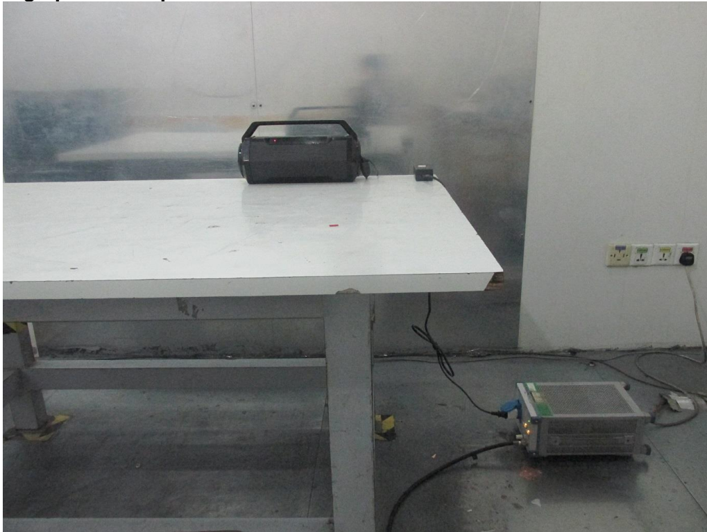
Photograph 4: Set-up for Radiated Emissions
