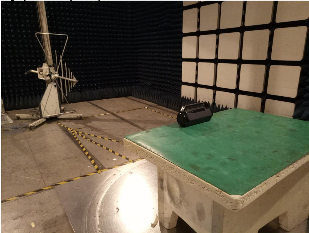
Photograph 2: Set-up for Spurious Emissions for 1 - 26.5GHz
