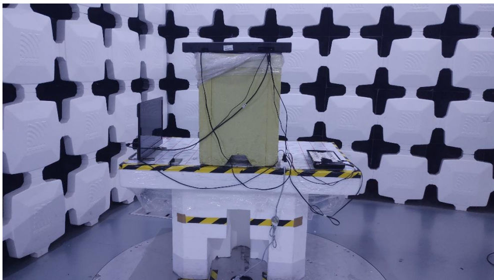
Back View (Above 1GHz)
