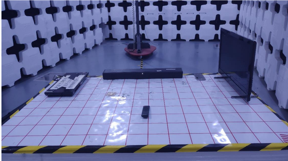
Front View (Below 1GHz)
