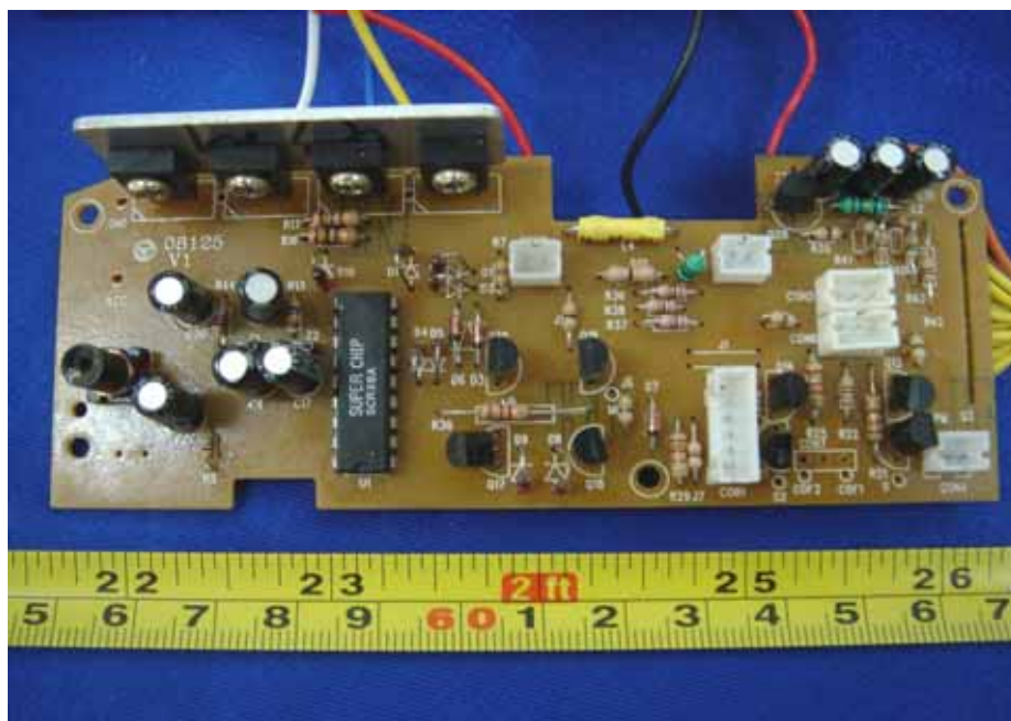
PCB 2- Component View
