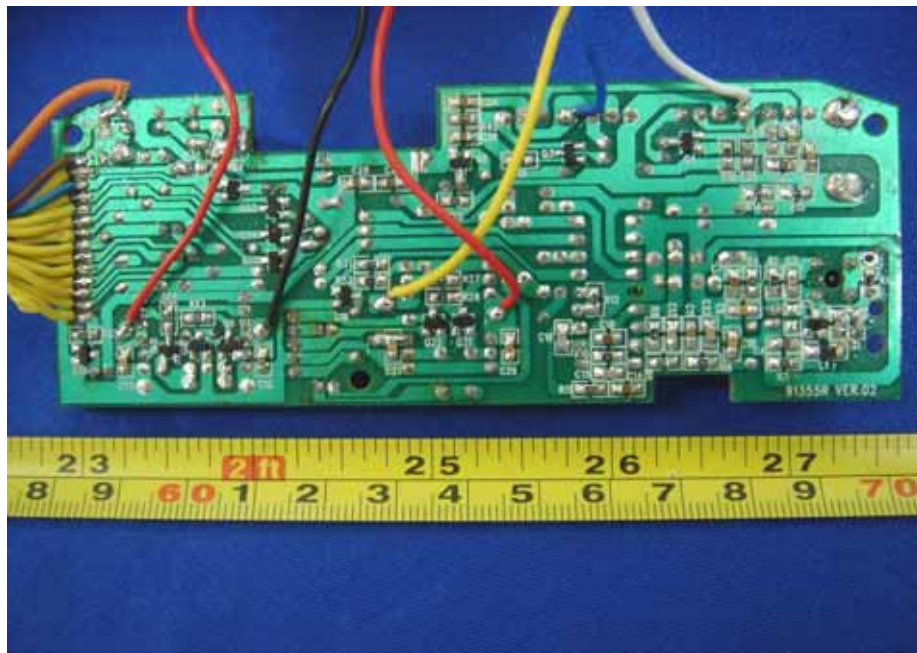
PCB2 - Solder View
