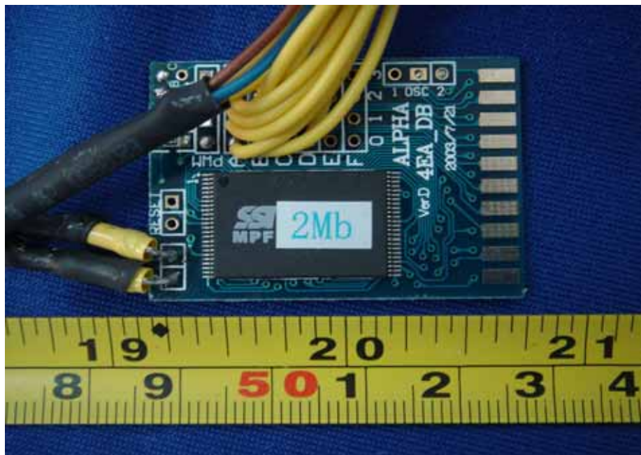
PCB 1- Component View
