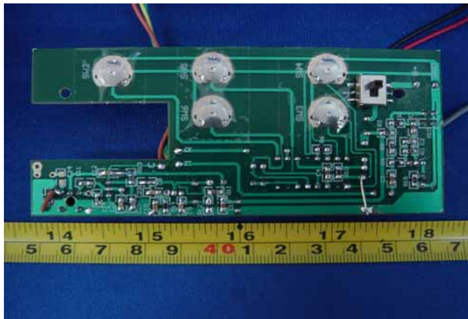
PCB - Solder View
