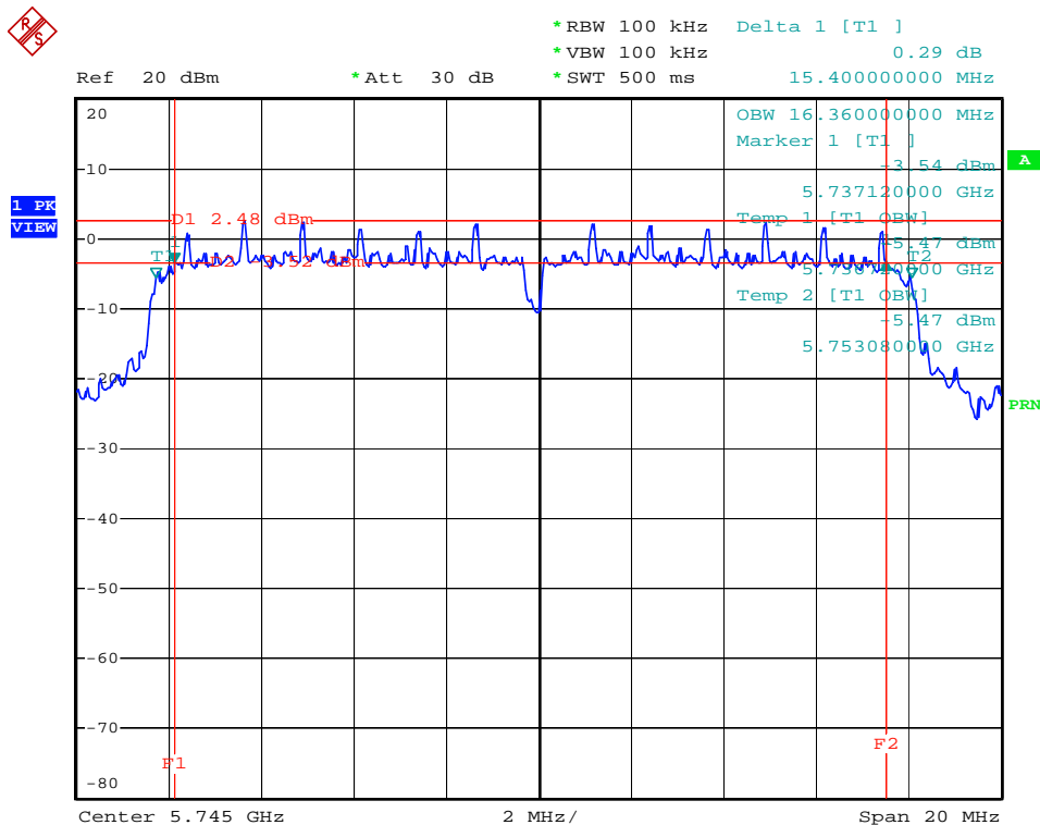
6 dB Bandwidth Plot on Configuration IEEE 802.11a / 5745 MHz
