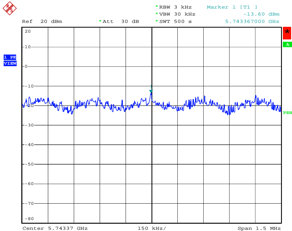
Power Density Plot on Configuration IEEE 802.11a / 5745 MHz
