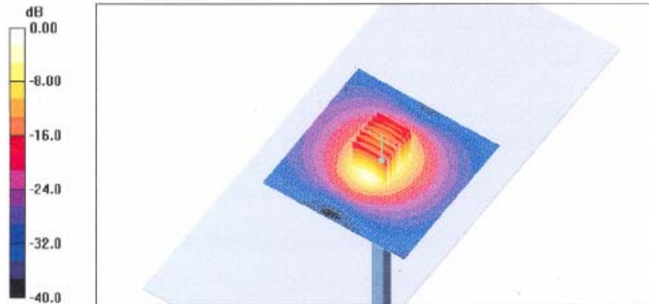
0 dB = 15.5mW/g
