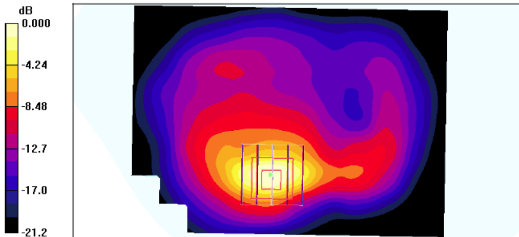
0 dB = 0.885mW/g
