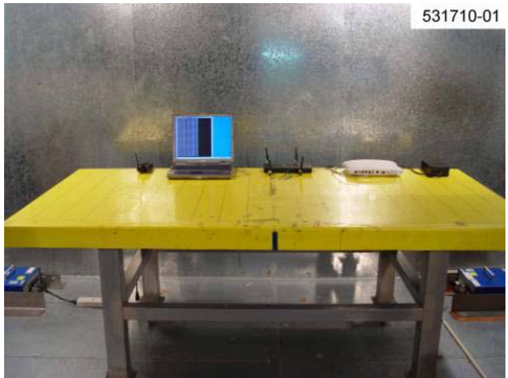
FRONT VIEW (Metallic Housing WASP-5100)
