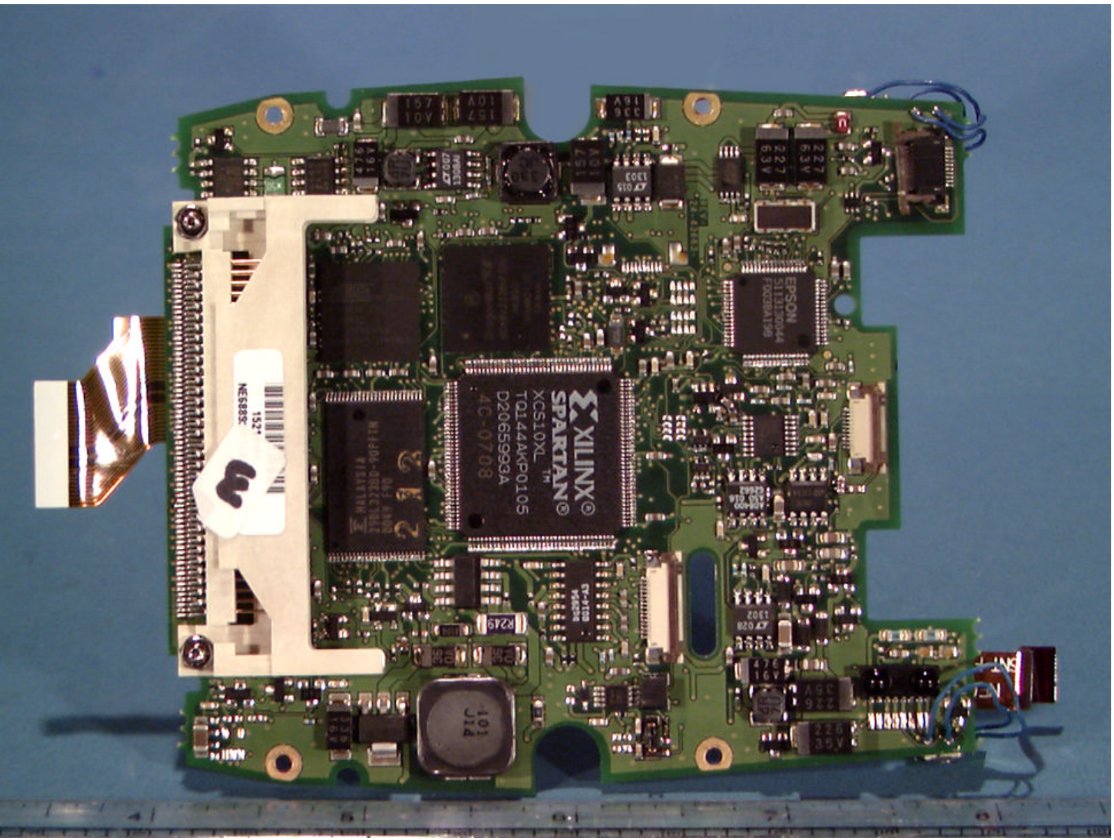
© 2001 PCTEST Lab SYMBOL FCC ID: H9PSP1833 (TX 824-849MHz) NVLAP Lab Code: 100431-0 Cellular PDA WAN Terminal w/ Integrated CDPD Radio Modem
