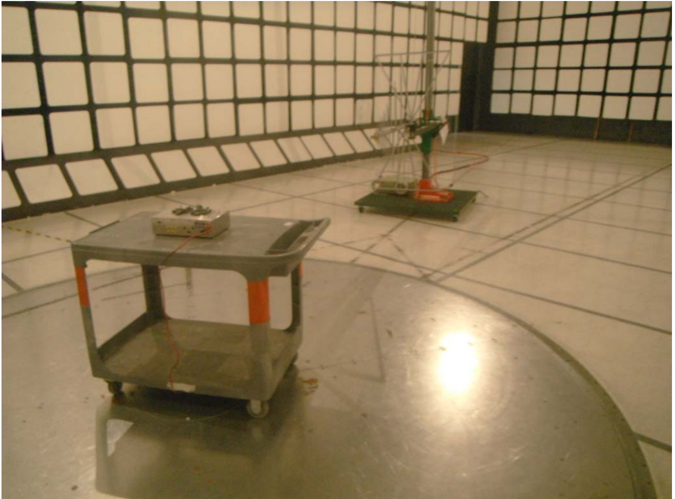
Radiated Emissions at 3 m, 30 - 1000 MHz Orthogonal Position 1
