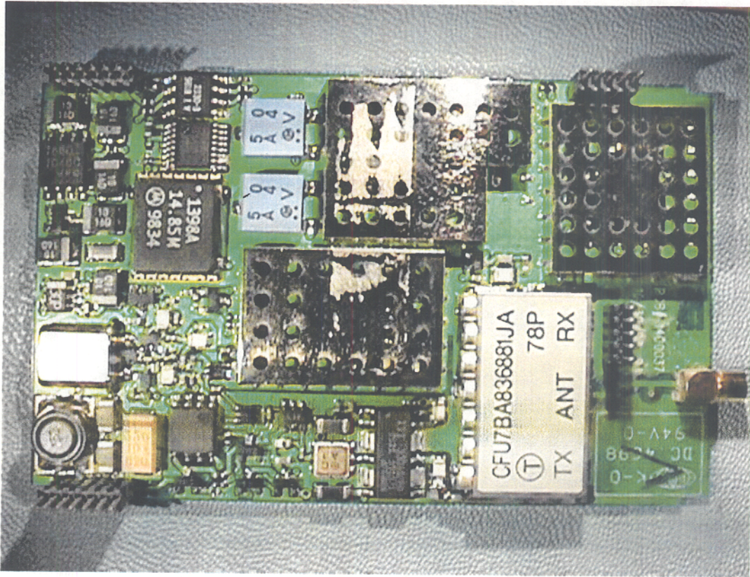
Figure3:ModemInternalView–RadioBoardTopSide
