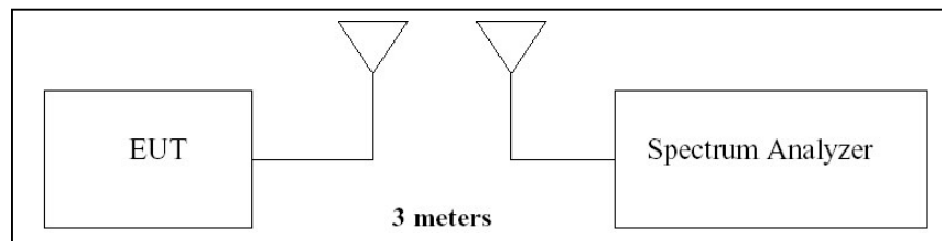
Figure A-1. Test Instrument & Measurement Setup
