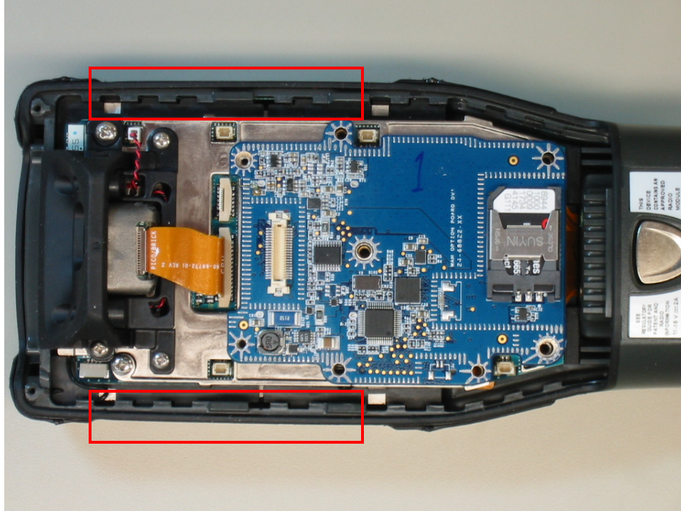
RLAN Antenna locations (in side of housing)
