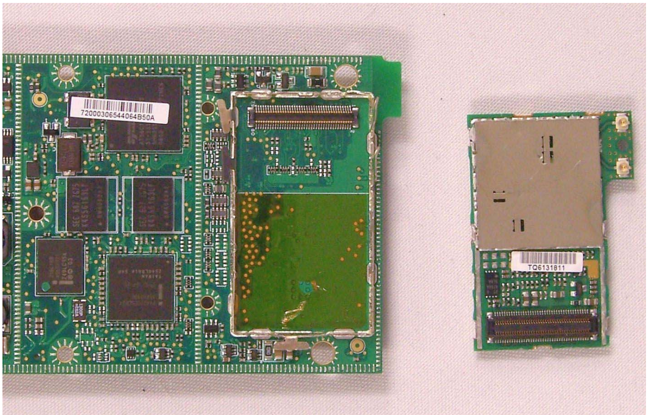
Main Board with WLAN (FCC ID: H9P2121160) Removed
