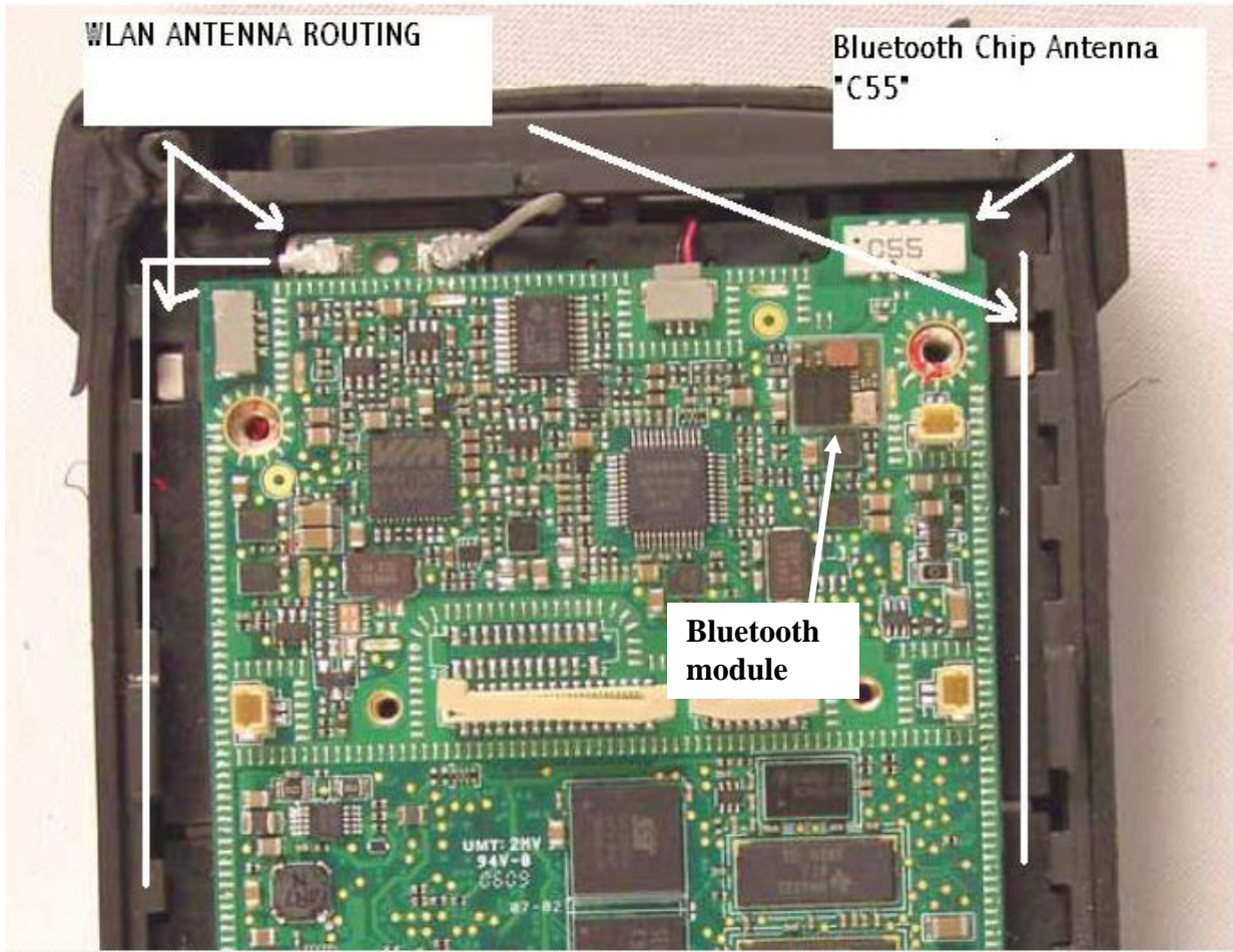
Main Board with WLAN (FCC ID: H9P2121160) Removed
