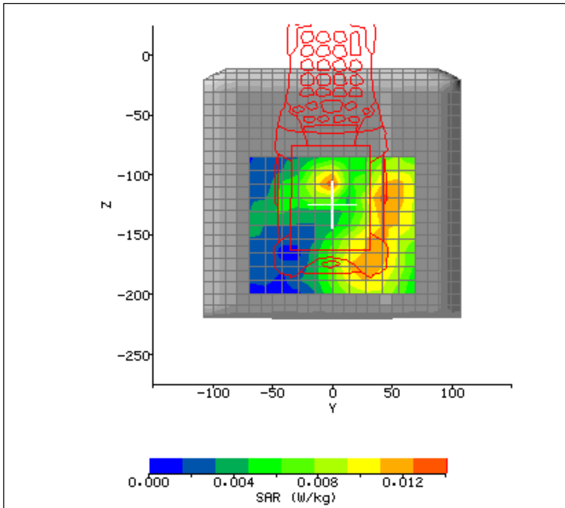
Figure 4 – Co-located SAR located in the centre at Belt Clip Location was shown to less than that of the Bluetooth Radio and therefore disregarded.
