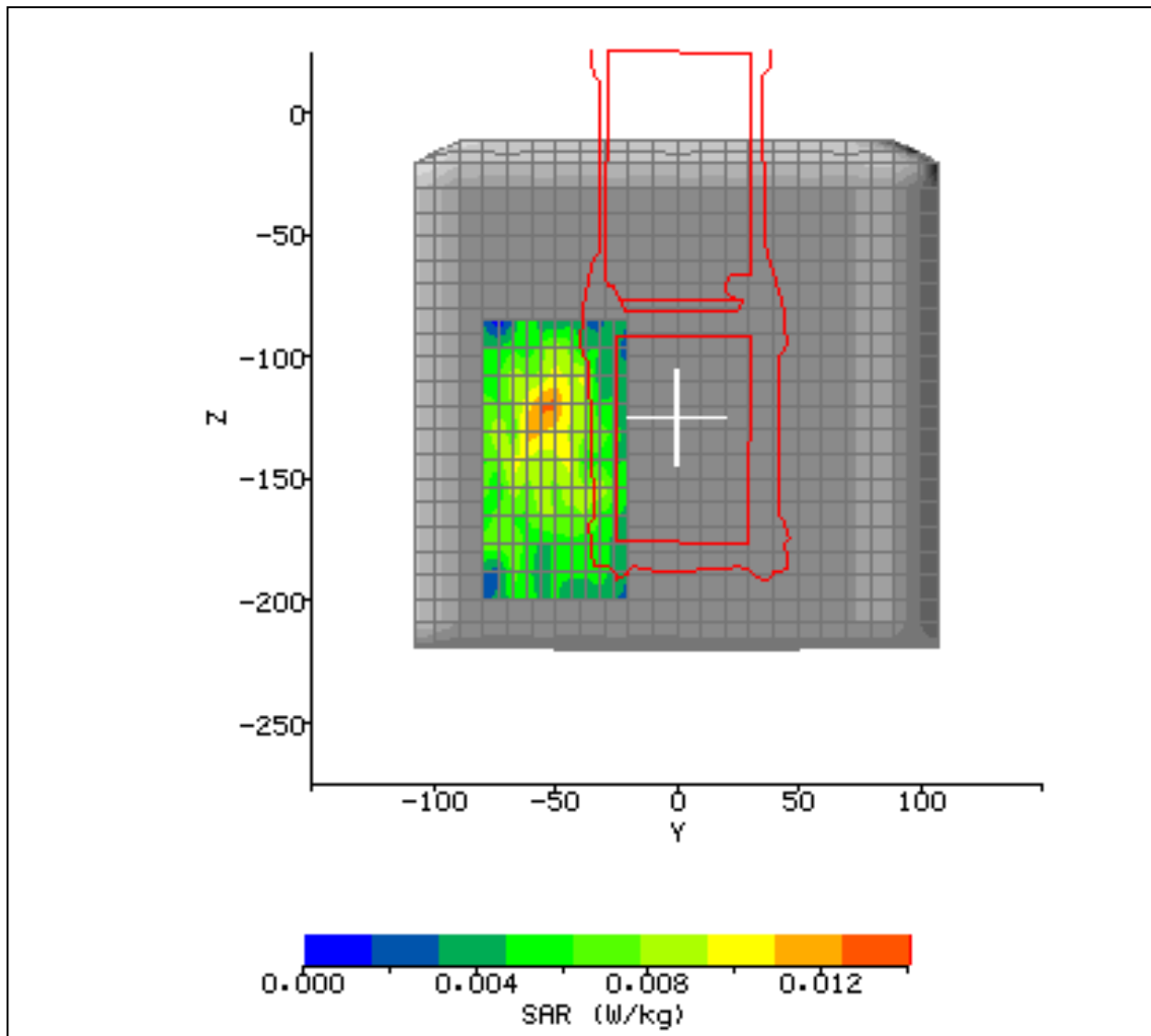
Figure 10 – Third High Energy Area, WLAN Radio
