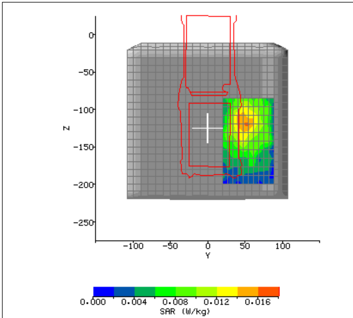
Figure 9 – Second High Energy Area, Bluetooth Radio
