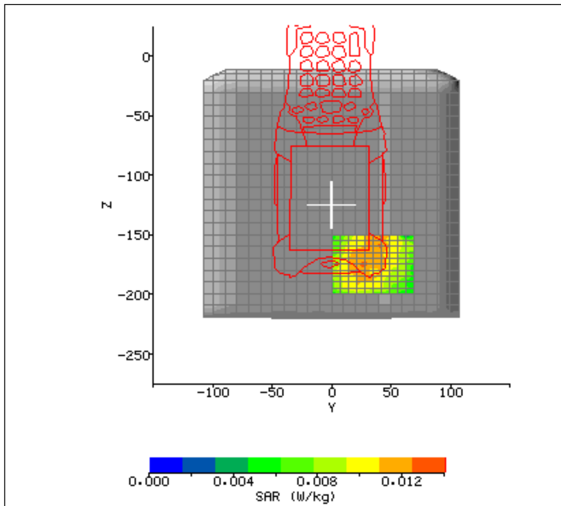
Figure 5 – Second High Energy Area as identified in Figure 4 (GPRS Radio).
