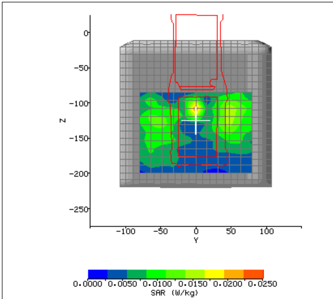
Figure 8 – First High energy area located in the centre co-located SAR at Belt Clip Location
