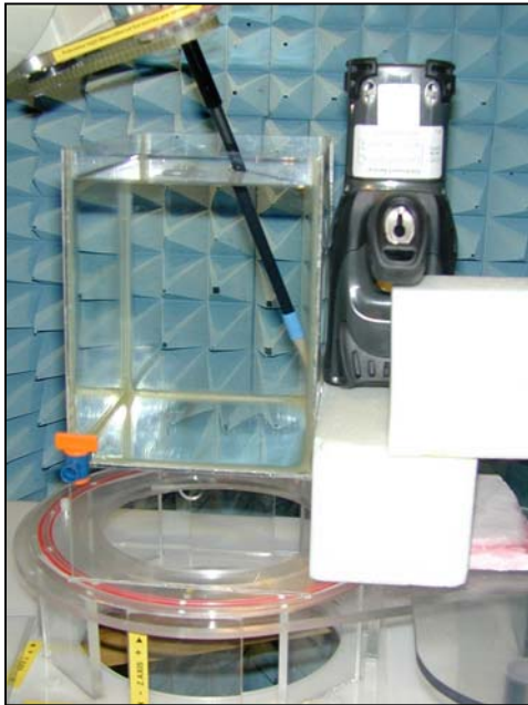
Figure 27. Positional photograph of MC9050 Left-Hand side in Touch Position
