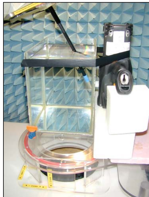
Figure 30. Positional photograph MC9050 Left-Hand side in 1.0 cm spacing
