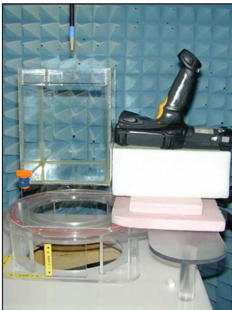
Figure 29. Positional photograph MC9050 Front End on Facing Touch Position
