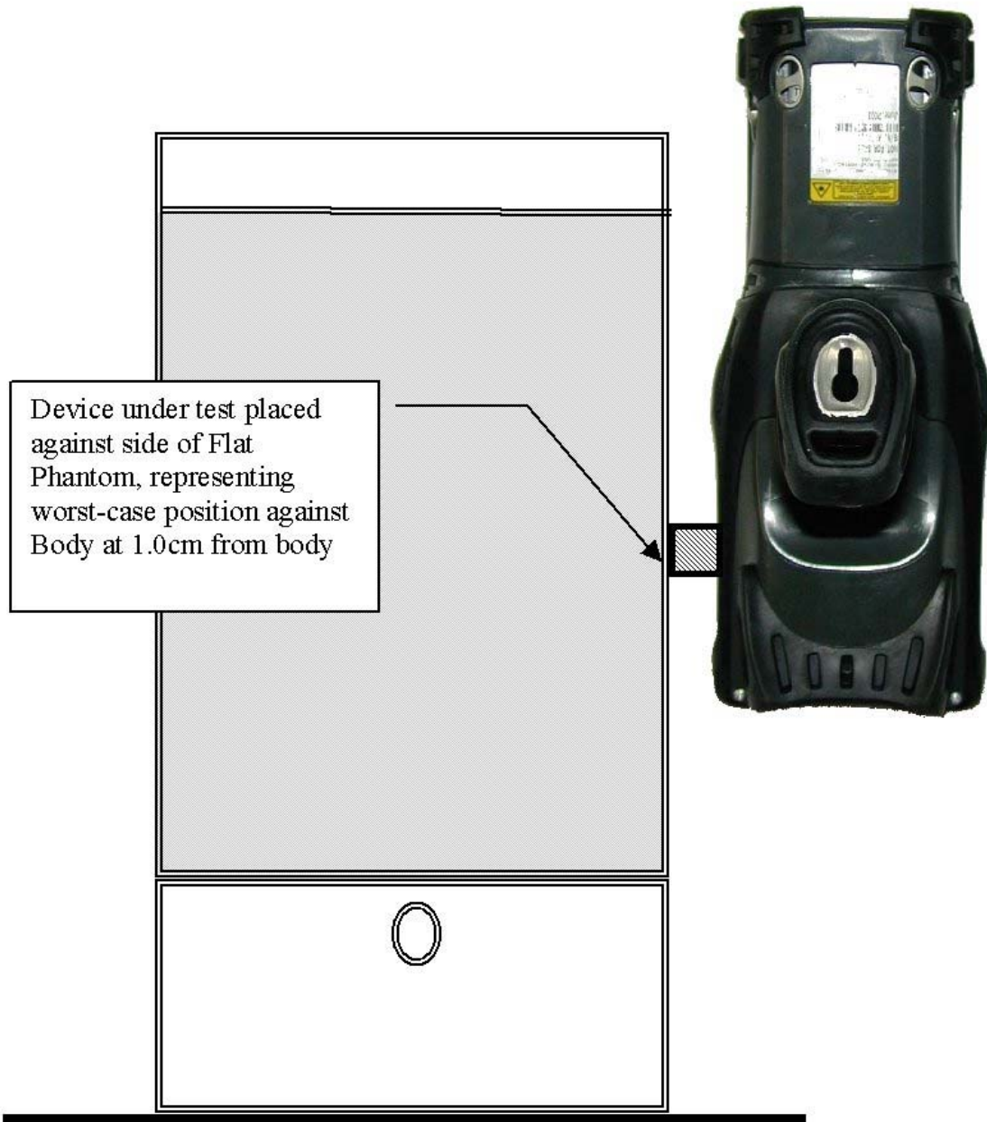
Figure 17. – 1.0 cm separation; Left hand side.
