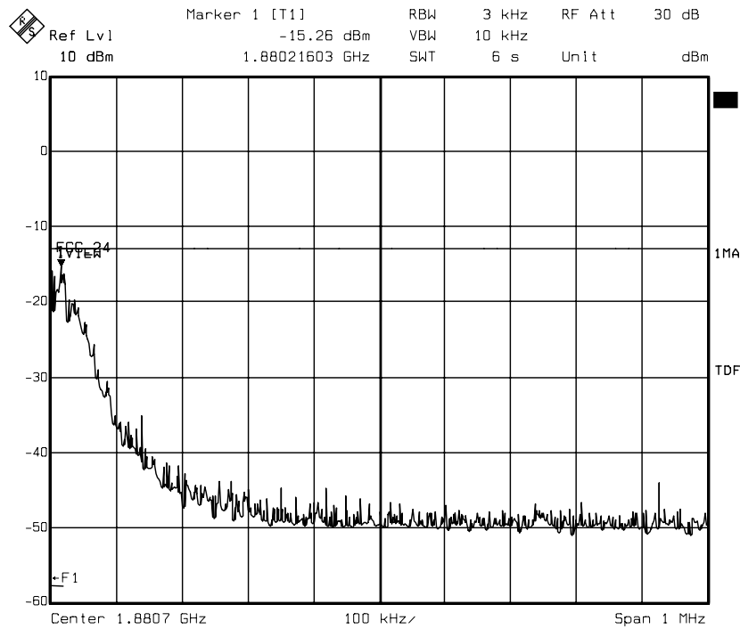
diagram 8.26: carrier on channel 661 (1880 MHz), TCH mode
