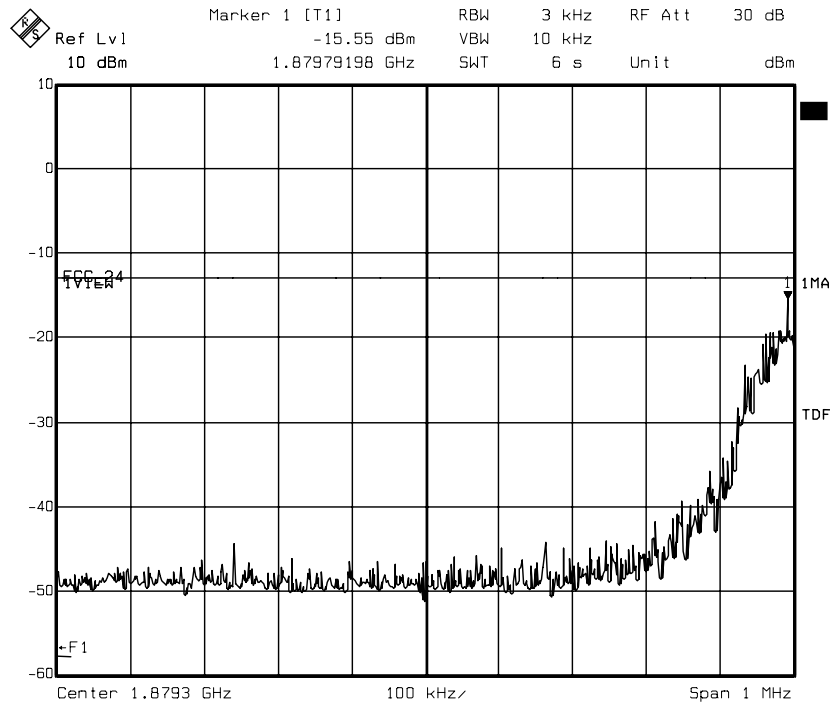
diagram 8.25: carrier on channel 661 (1880 MHz), TCH mode
