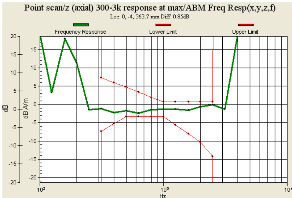
Figure 9.2: Frequency Response of CDMA2000 Cellular for Ch384
