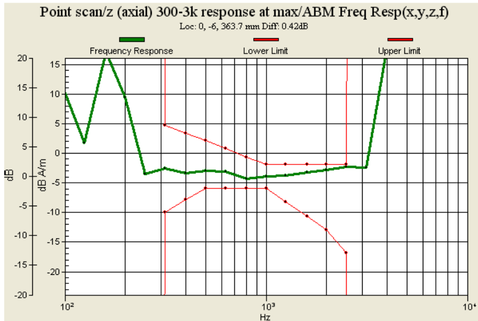
Figure 9.5: Frequency Response of CDMA2000 PCS for Ch600
