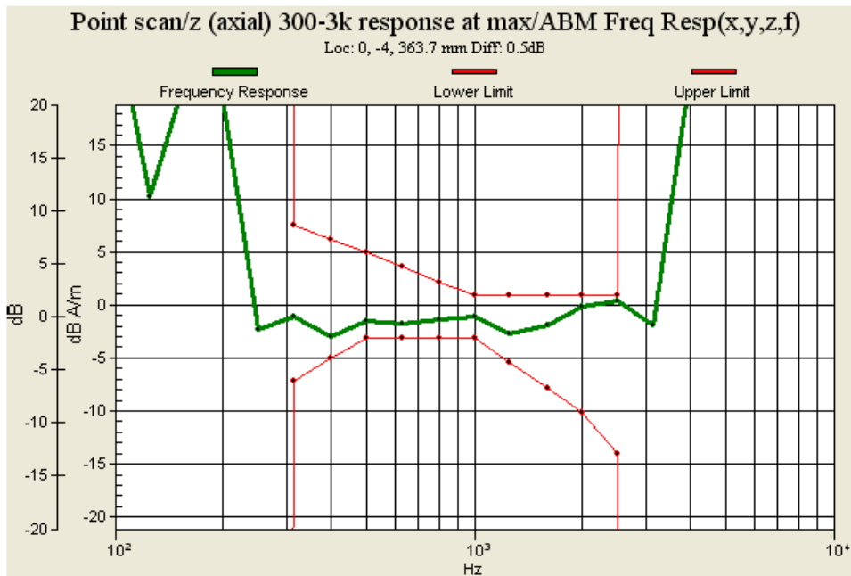
Figure 9.3: Frequency Response of CDMA2000 Cellular for Ch777
