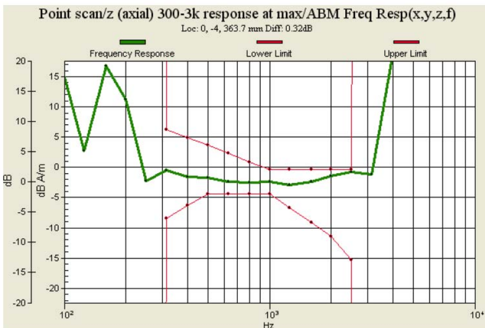
Figure 9.8: Frequency Response of CDMA2000 PCS for Ch25
