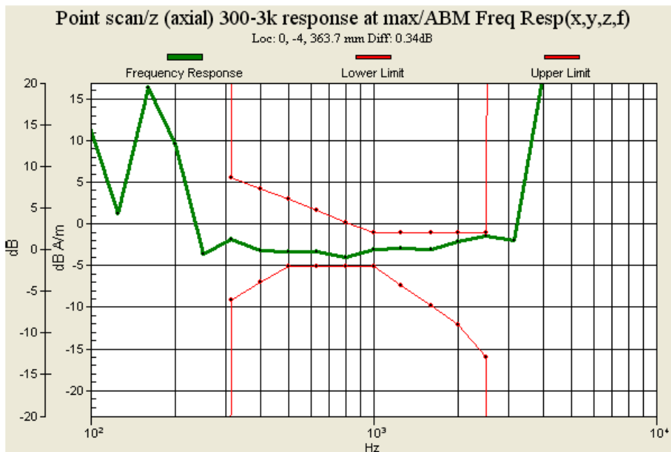
Figure 9.4: Frequency Response of CDMA2000 PCS for Ch25
