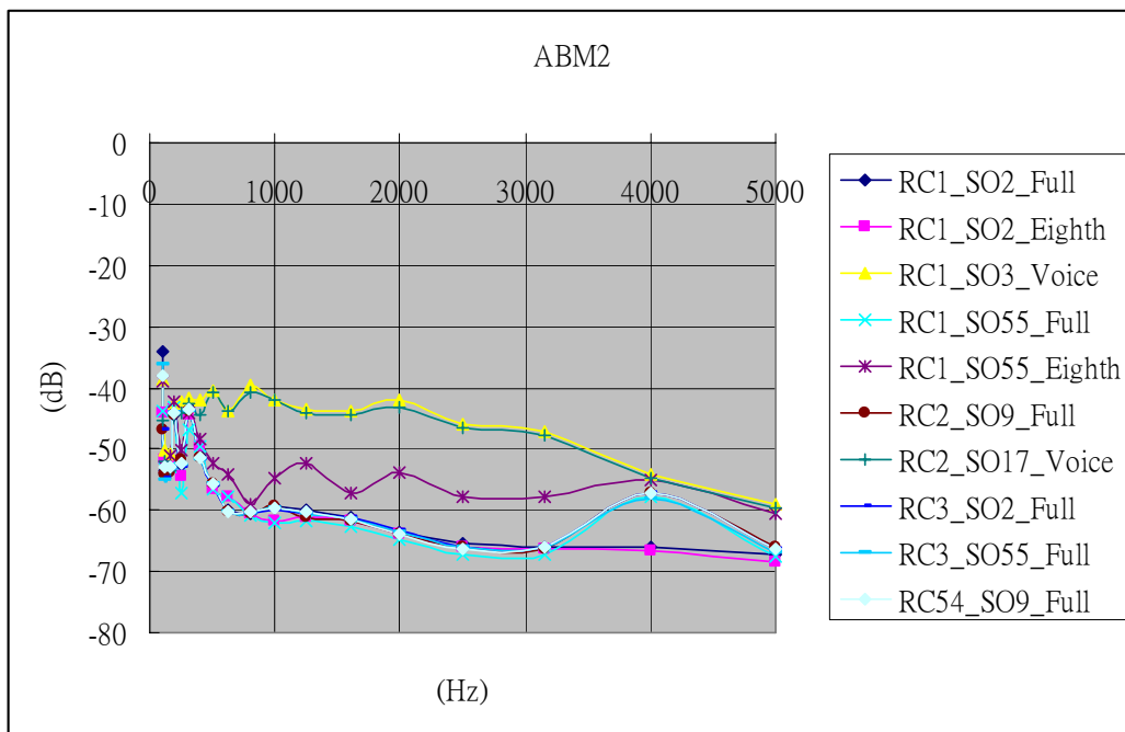
Figure 5.10: Vocoder Analysis for ABM Noise
