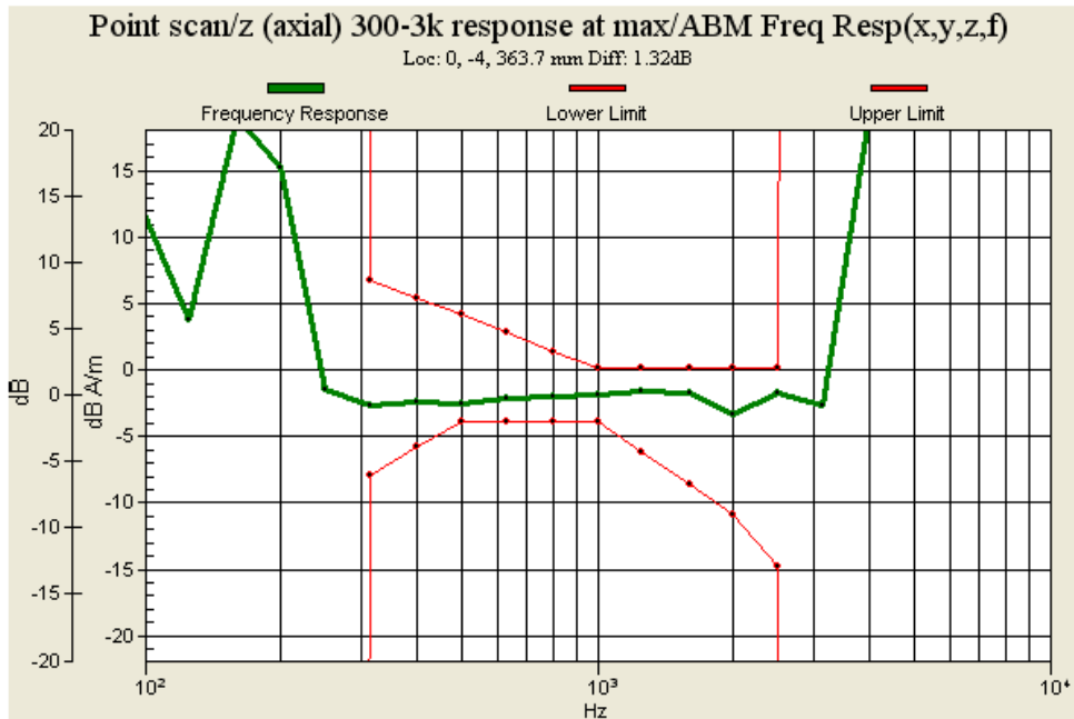
Figure 9.1: Frequency Response of CDMA2000 Cellular for Ch1013
