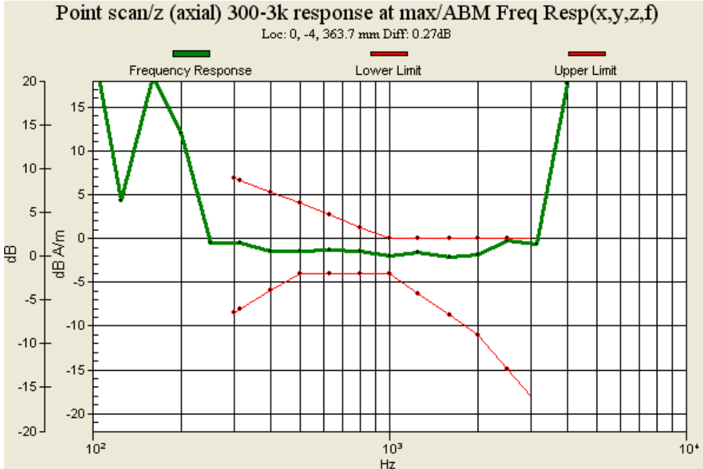
Fig. 9.8: Frequency Response of CDMA2000 PCS Ch1175 for Sample 1
