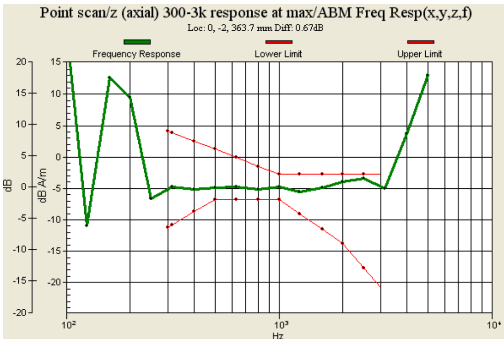
Fig. 9.8: Frequency Response of CDMA2000 PCS Ch25 for Sample 1
