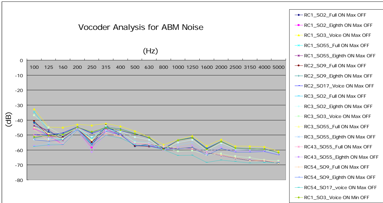
Fig. 5.10: Vocoder Analysis for ABM Noise
