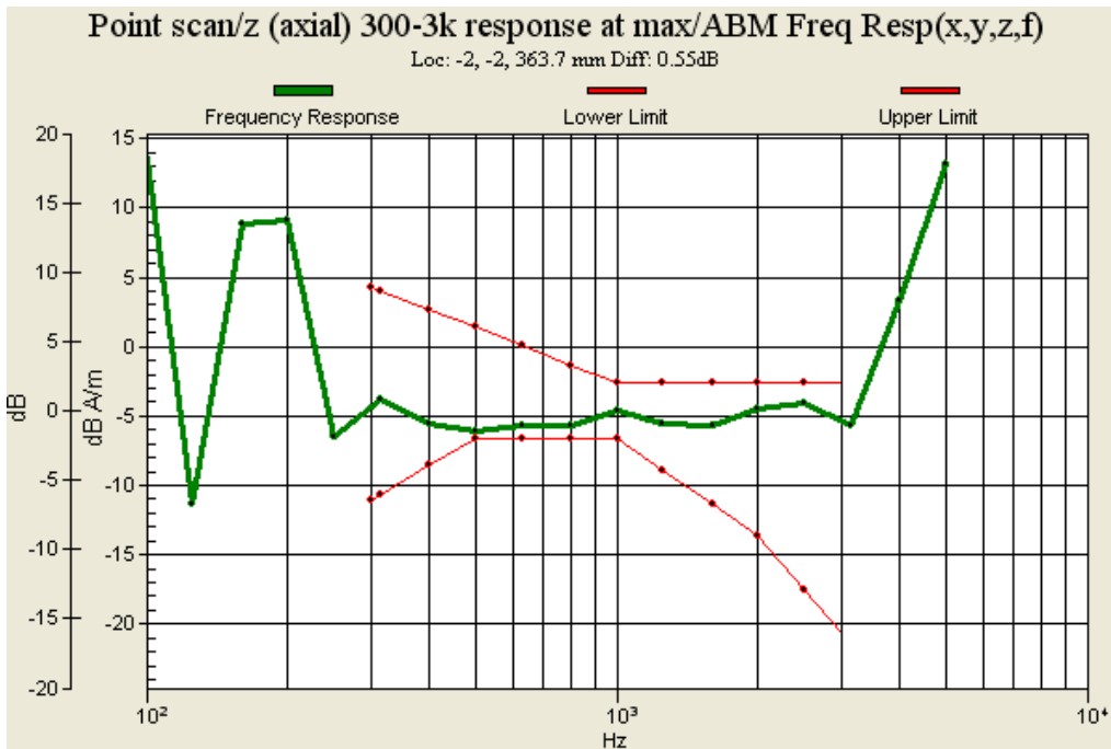
Fig. 9.1: Frequency Response of CDMA2000 Cellular Ch1013 for Sample 2
