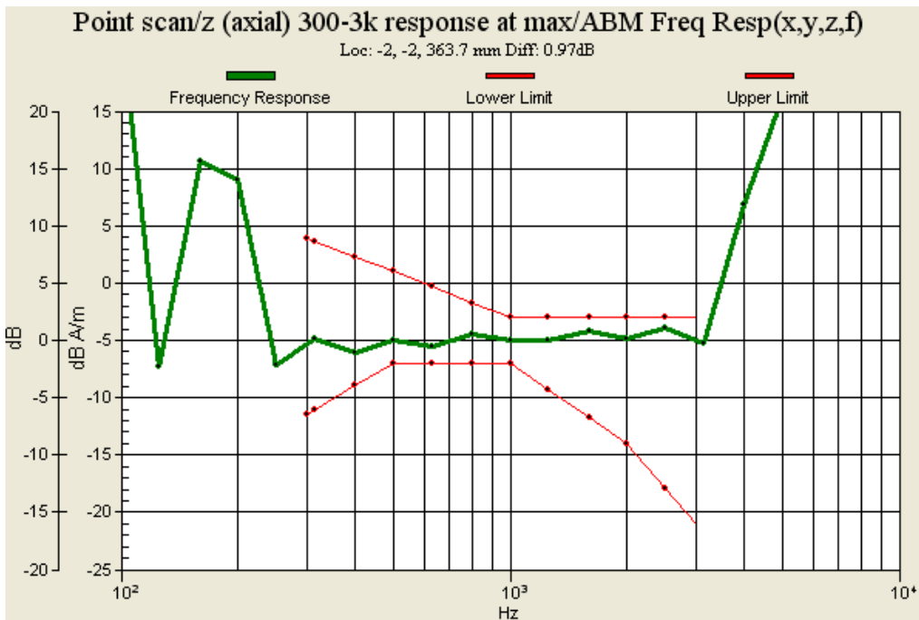
Fig. 9.3: Frequency Response of CDMA2000 Cellular Ch777 for Sample 2
