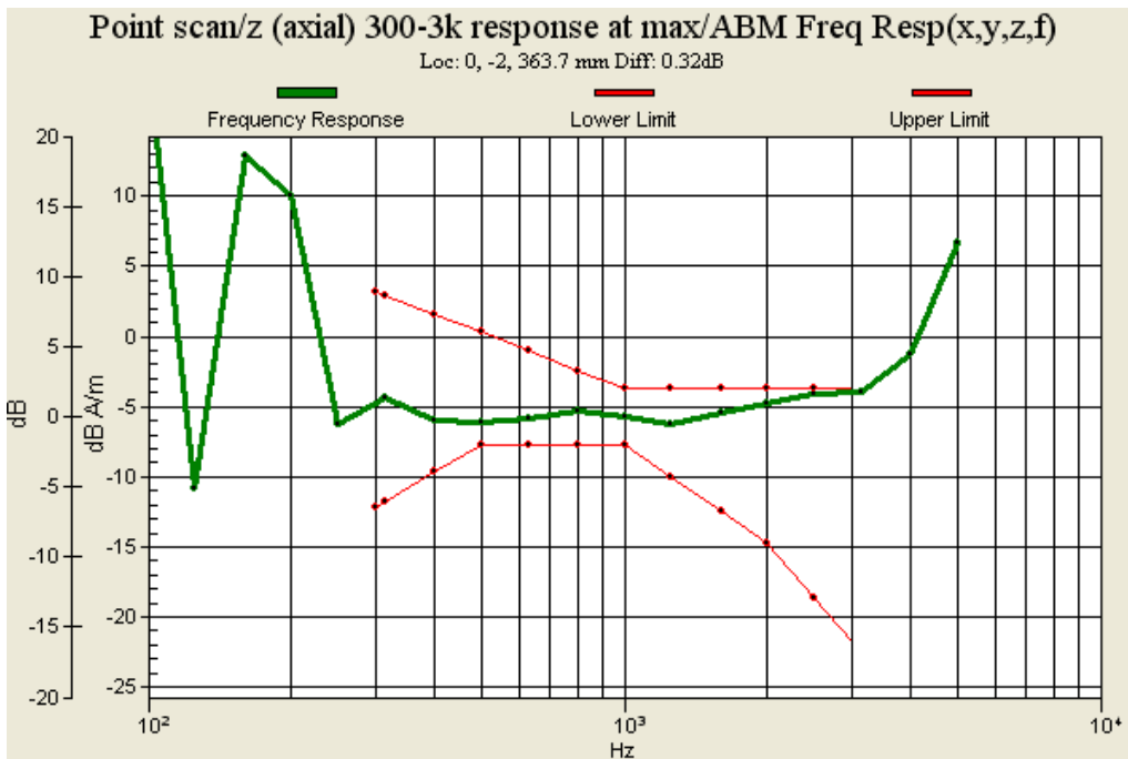
Fig. 9.7: Frequency Response of CDMA2000 PCS Ch1175 for Sample 2
