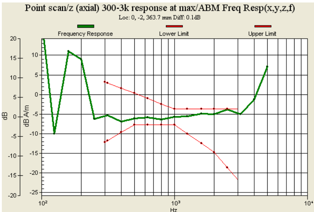
Fig. 9.4: Frequency Response of CDMA2000 Cellular Ch777 for Sample 1
