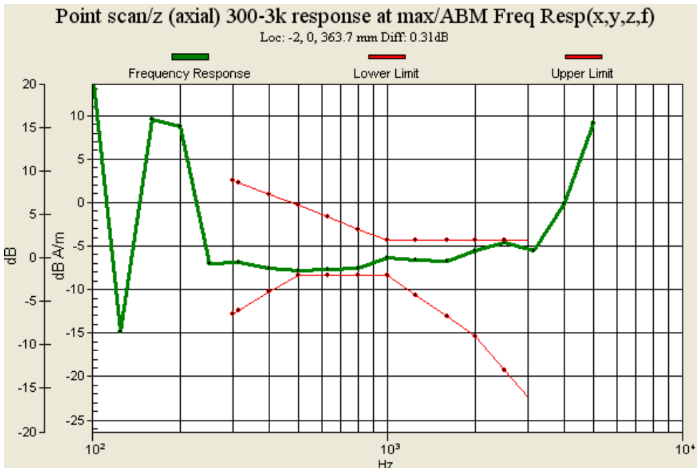
Fig. 9.2: Frequency Response of CDMA2000 Cellular Ch384 for Sample 2
