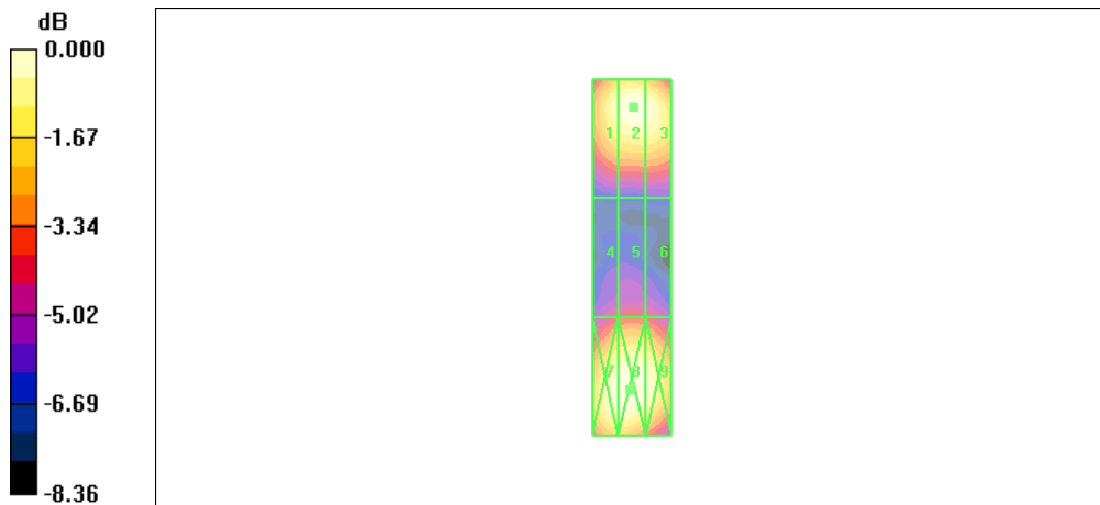
0 dB = 147.9V/m
