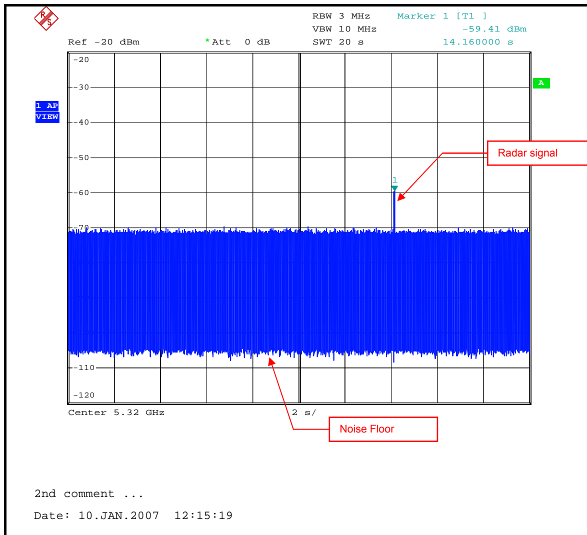
Radar Signal 1
