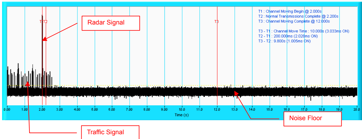
Radar signal 1
