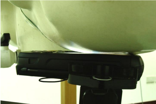
Left Cheek - DUT with Battery 1 + Scanner 2 + Keypad 1
