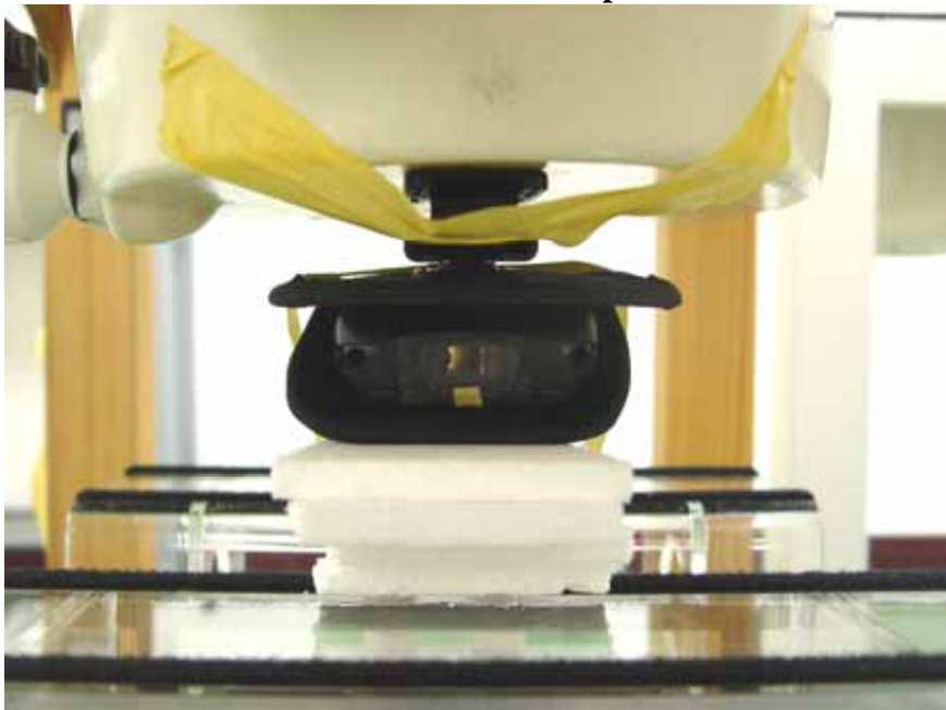
EUT with 1D Scanner and Holster 2 Face with 0cm Gap
