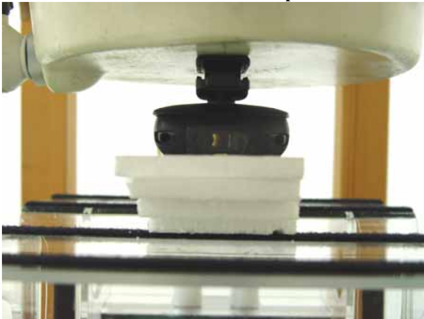
EUT with 1D Scanner and Holster 1 Face with 0cm Gap
