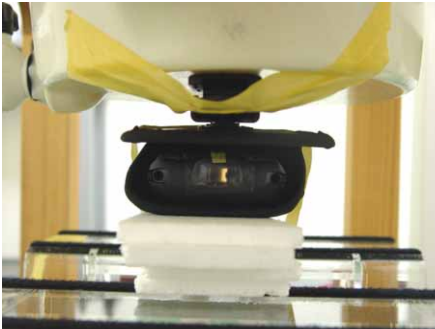
EUT with 1D Scanner and Holster 2 Bottom with 0cm Gap
