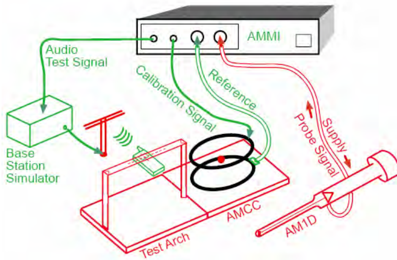
Figure 4. T-Coil Measurement system
