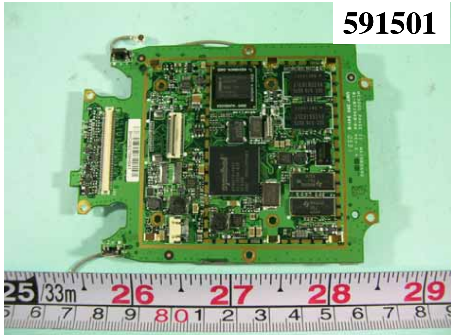
Main Board
