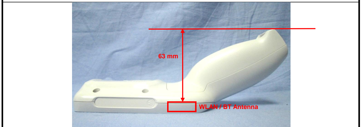
EUT Side View
