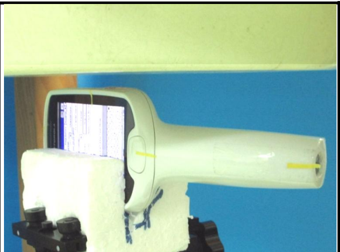
Body-worn Mode, ANT Side of EUT with 1.0 cm Gap
