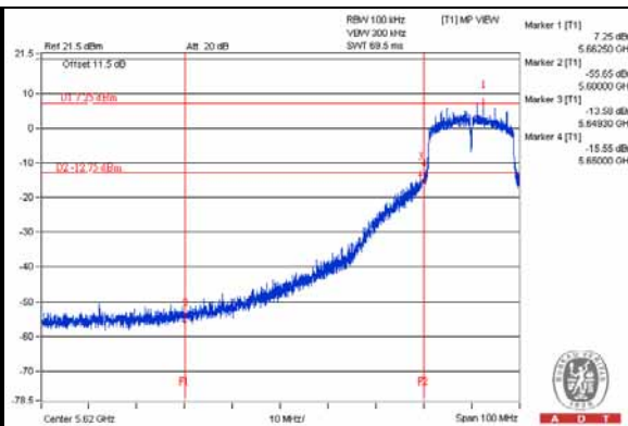
802.11n (HT20) OFDM MODULATION (CH 132: 5660MHz)
