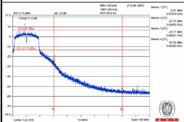
802.11n (HT20) OFDM MODULATION (CH 116: 5580MHz)
