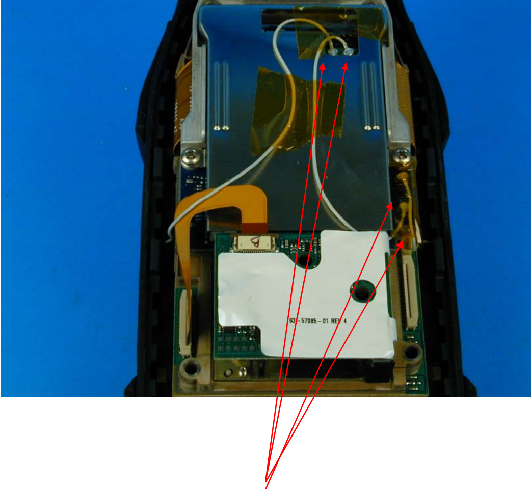
Antenna Connection points for 2.4GHz RLAN and Bluetooth
