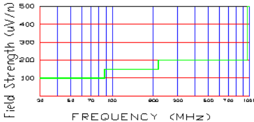
Figure B-11. Radiated limits at 3 meters.
