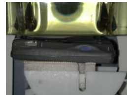
Figure 14.2 Hand SAR Test Setup -- w/out Holster --
