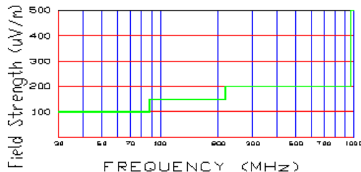
Figure A-2. Radiated limits at 3 meters.
