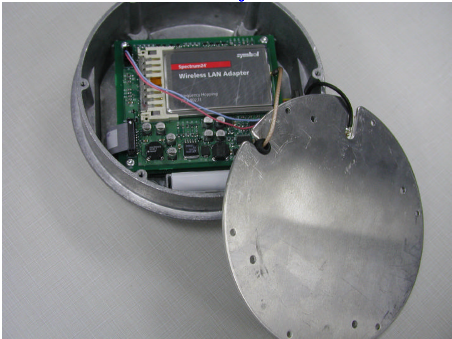
The Symbol LA-3021-100-US radio Shown inside the housing in which it was tested
