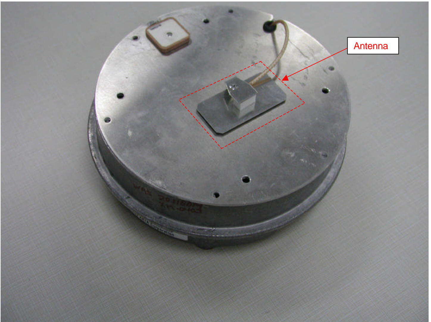
Maxrad mn: Z1370 Inverted F, 3 dBi Gain Antenna
