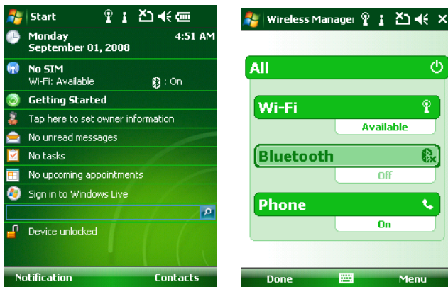
Figure 4-1 Disable Bluetooth
