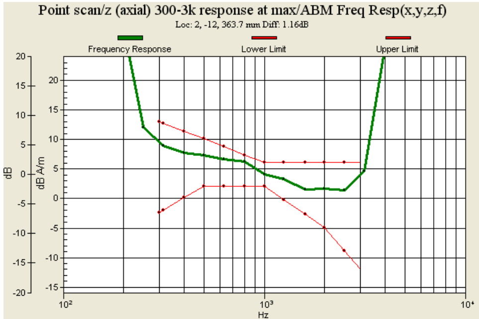
Fig. 9.5 Frequency Response of PCS1900 for Ch512
