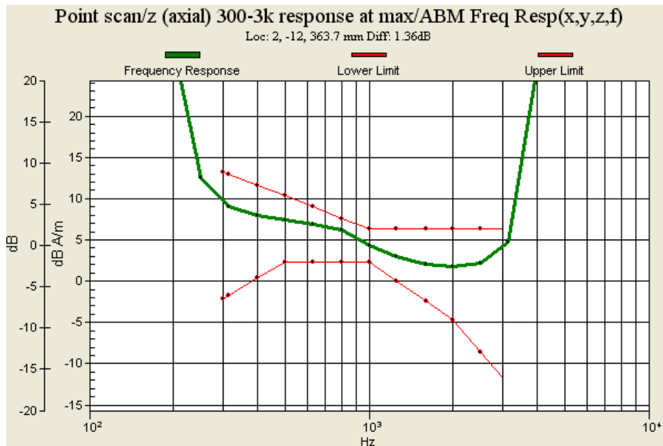
Fig. 9.2 Frequency Response of GSM850 for Ch189
