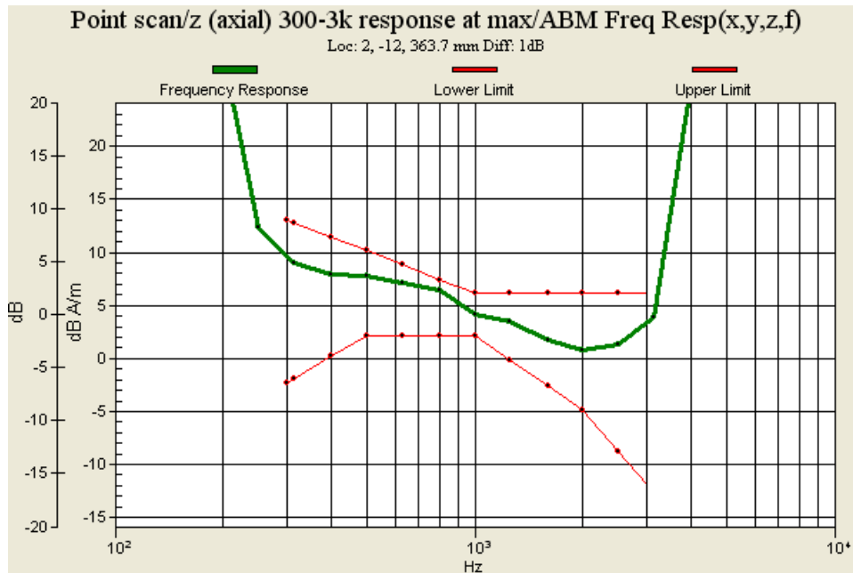
Fig. 9.1 Frequency Response of GSM850 for Ch128
