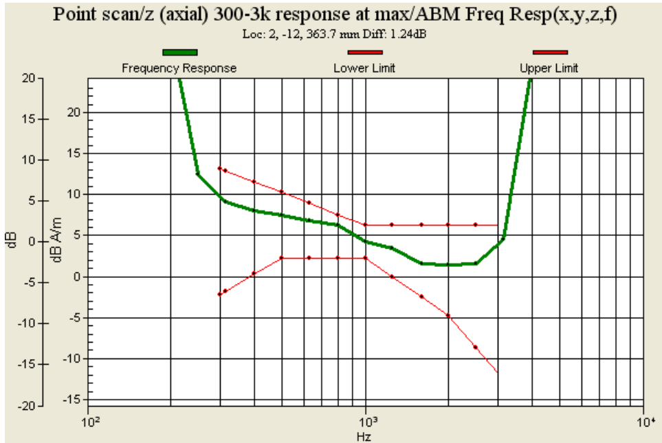
Fig. 9.3 Frequency Response of GSM850 for Ch251
