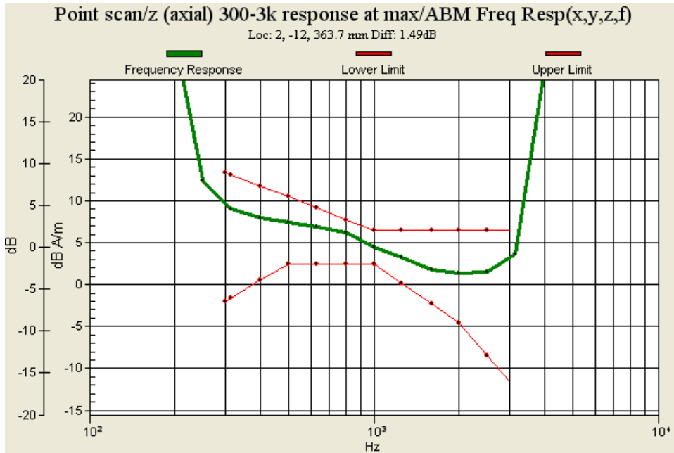
Fig. 9.7 Frequency Response of PCS1900 for Ch810
