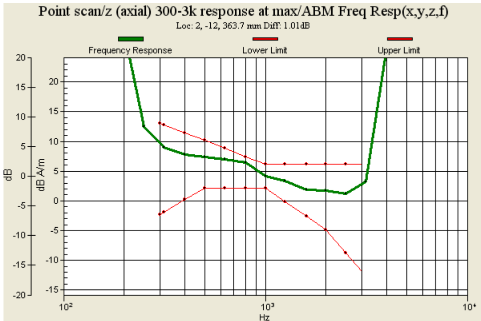
Fig. 9.6 Frequency Response of PCS1900 for Ch661
